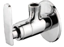
Cat Code 2003 Angular Stop Cock With Wall Flange M.R.P. : 530/-
